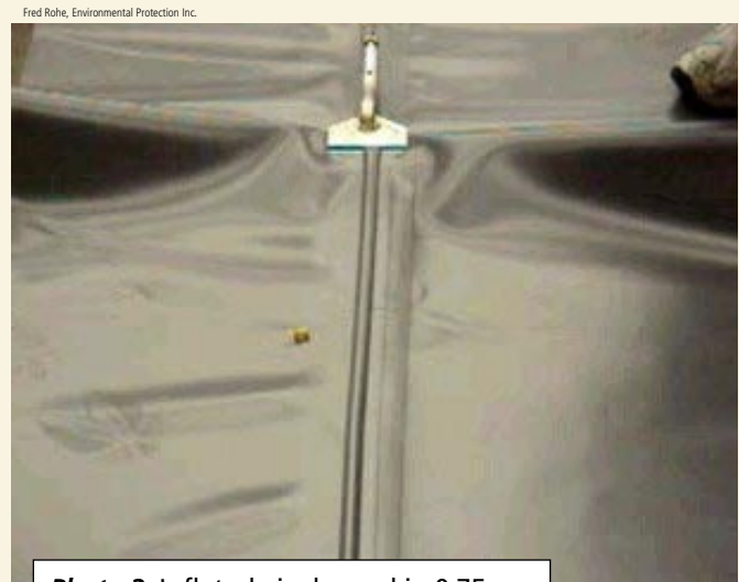
Photo 2. Inflated air channel in 0.75 mm (30 mil) geomembrane in the field.
